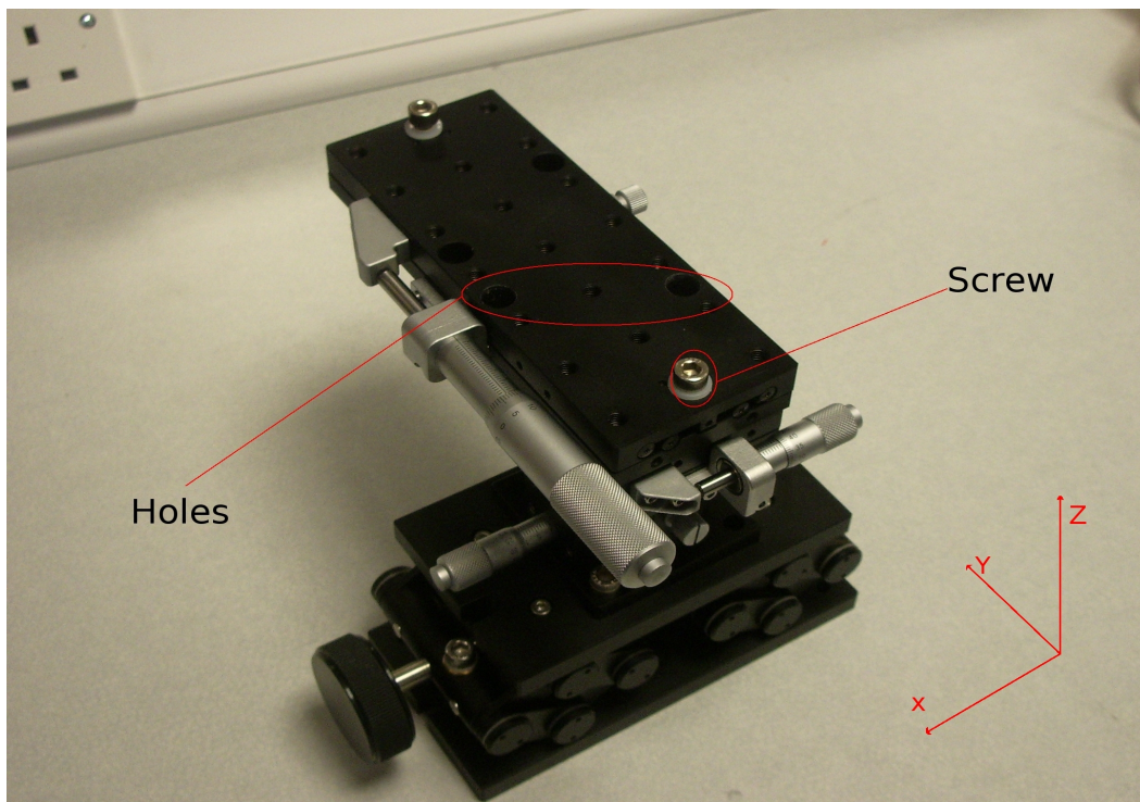
Figure 14: Micropositioning stage
